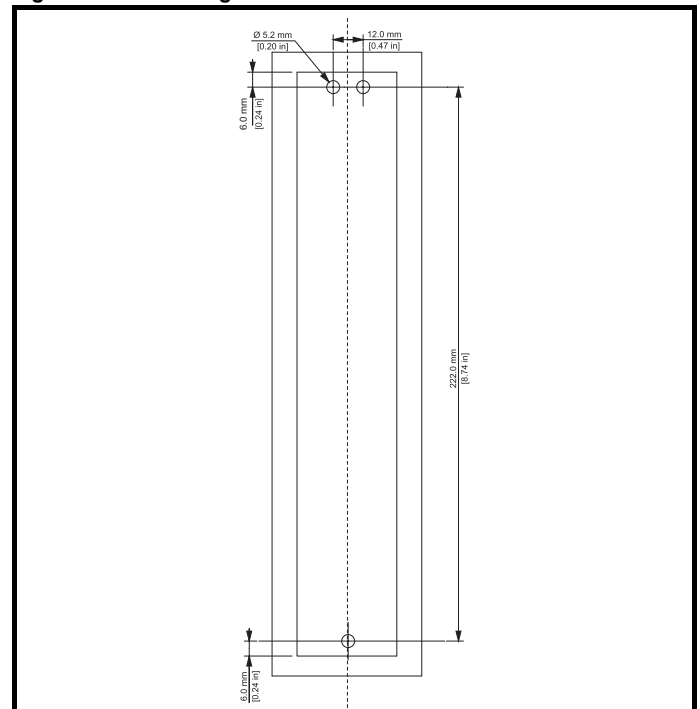
Figure 3-1 Mounting hole details
