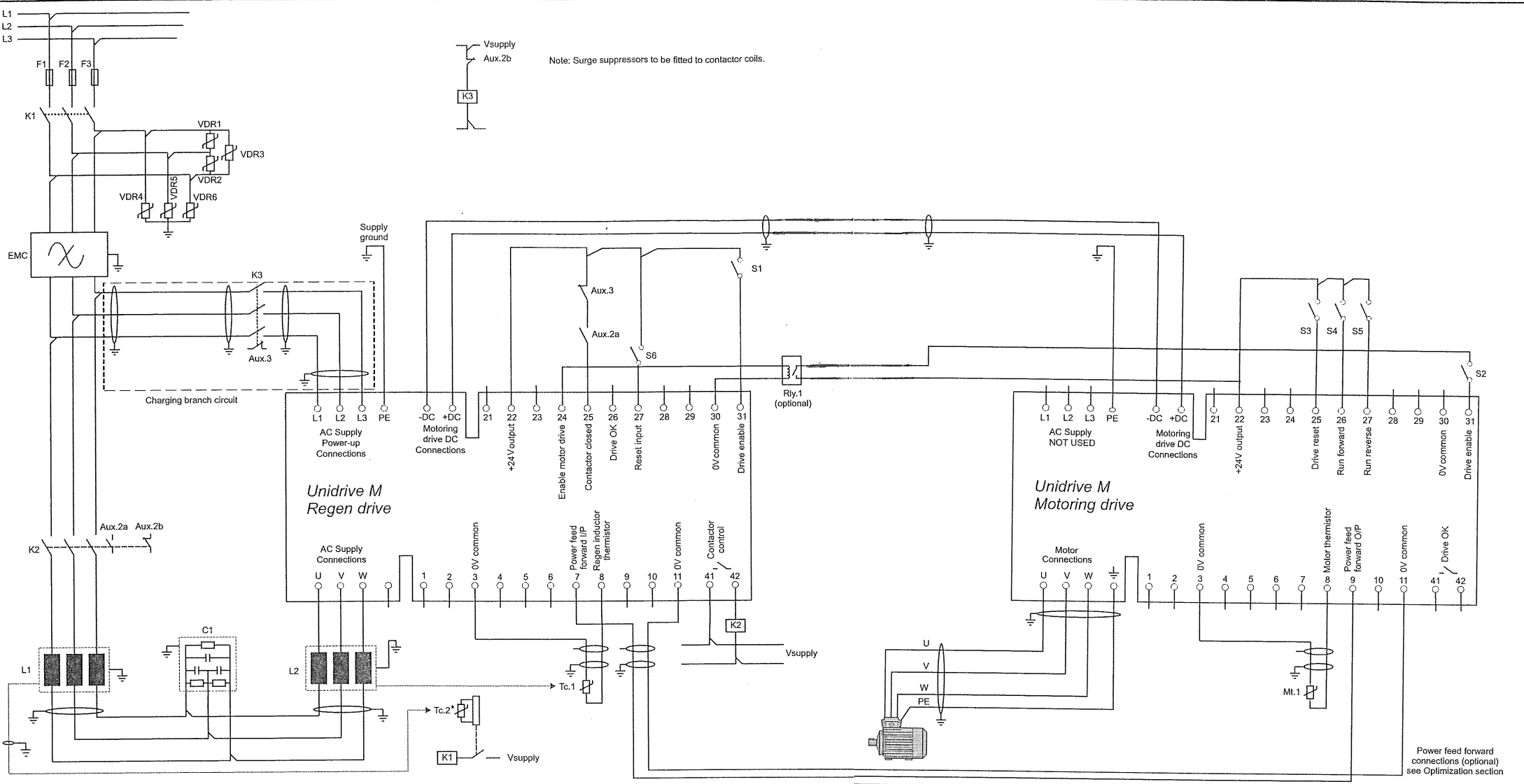
1-1 Power connections: Single Regen, single motoring system
